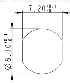
Panel Cut-out
